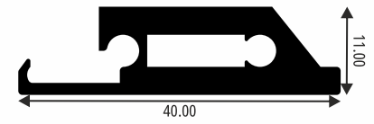
SH-2045 5MM X 40MM PROFILE
