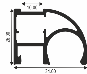
SH-2032 VERTICAL HANDLE
