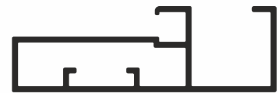
SH-2007 67MM HANDLE PROFILE
