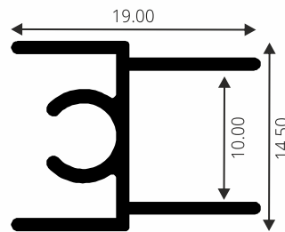
SH-2031 HORIZONTAL TOP PROFILE
