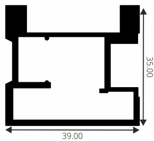
SH-2033 VERTICAL HANDLE
