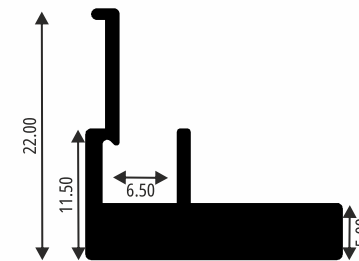
SH-2024 TOP / BOTTOM PROFILE 250 MM | 348 MM | 398 MM | 448 MM | 498 MM 548 MM | 598 MM | 748 MM | 898 MM
