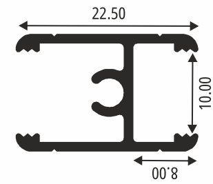
SH-2029 HORIZONTAL DIVIDING PROFILE
