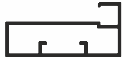
SH-2006 45MM FRAME PROFILE
