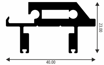
SH-2046 5MM X 40MM PROFILE
